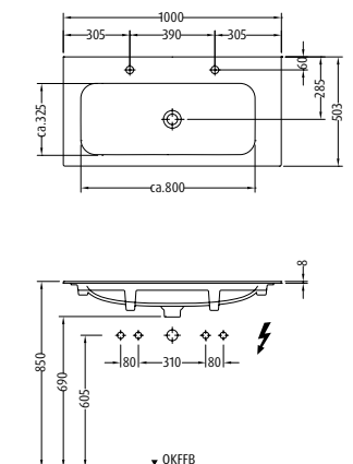
SL262/SL272
